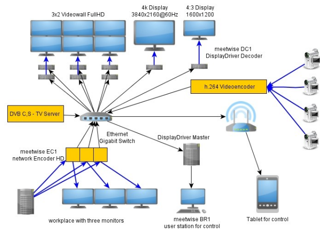
meetwise miniDisplayDriver distributed videowall example setup
